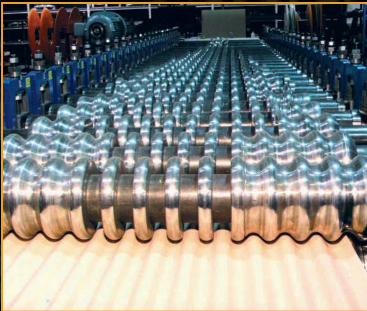
The IRONCLAD™ Panel Rollformer
